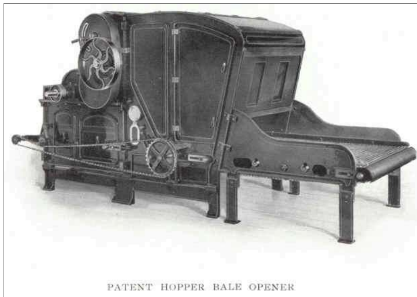
PATENT HOPPER BALE OPENER
