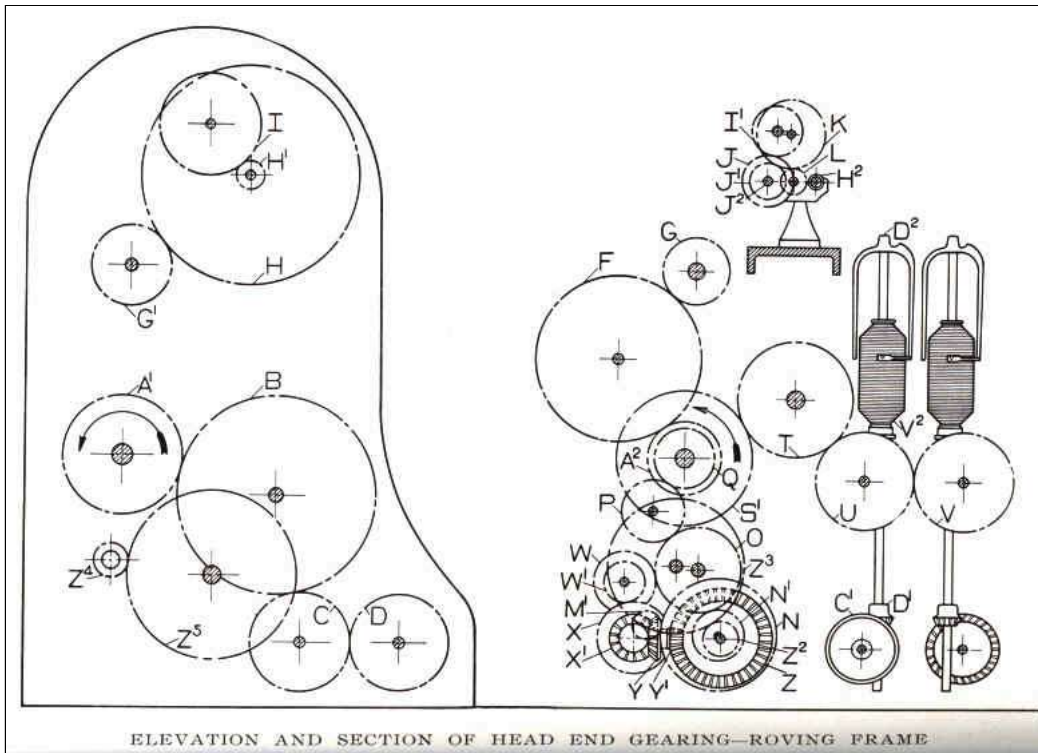
ELEVATION AND SECTION OF HEAD END GEARING—ROVING FRAME
