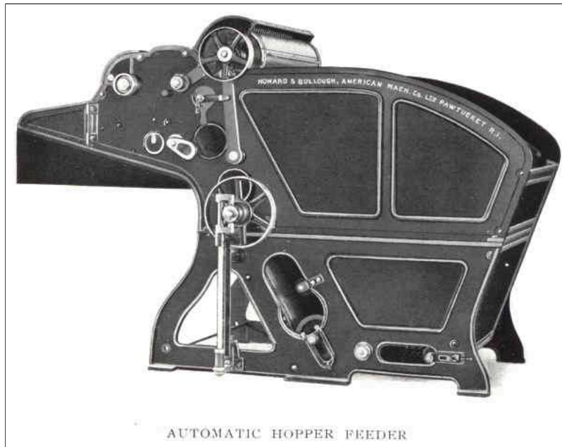
AUTOMATIC HOPPER FEEDER
