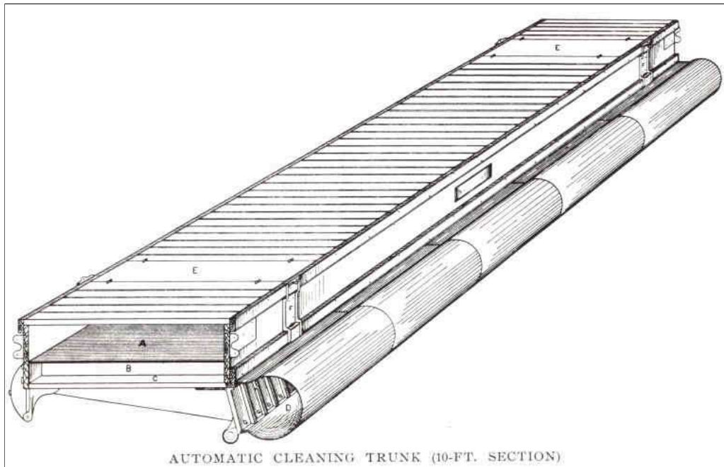
AUTOMATIC CLEANING TRUNK (10-FT. SECTION) AUTOMATIC CLEANING TRUNK (10-FT. SECTION)
