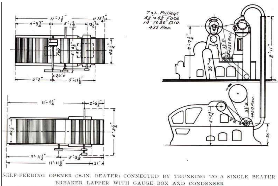
SELF-FEEDING OPENER (18-IN. BEATER) CONNECTED BY TRUNKING TO A SINGLE BEATER BREAKER LAPPER WITH GAUGE BOX AND CONDENSER
