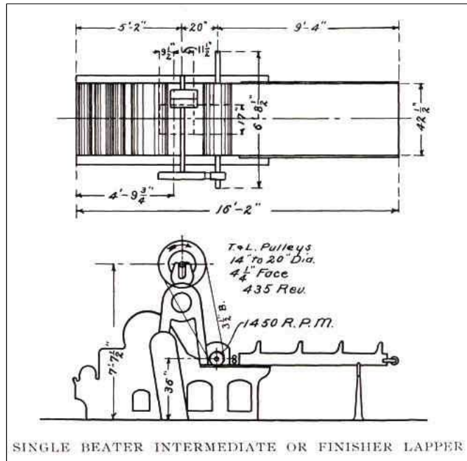
SINGLE BEATER INTERMEDIATE OR FINISHER LAPPER
