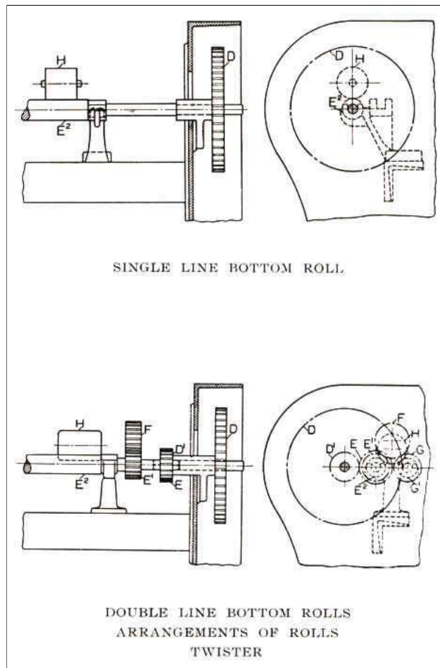
SINGLE LINE BOTTOM ROLL
