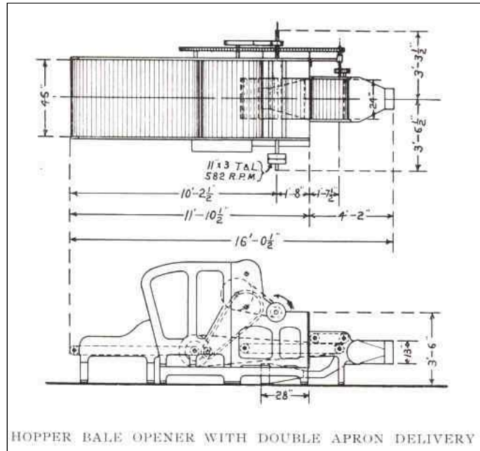
HOPPER BALE OPENER WITH DOUBLE APRON DELIVERY
