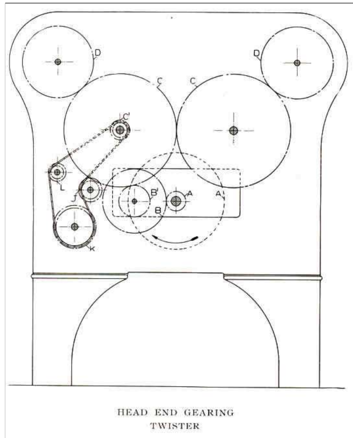
HEAD END GEARING TWISTER
