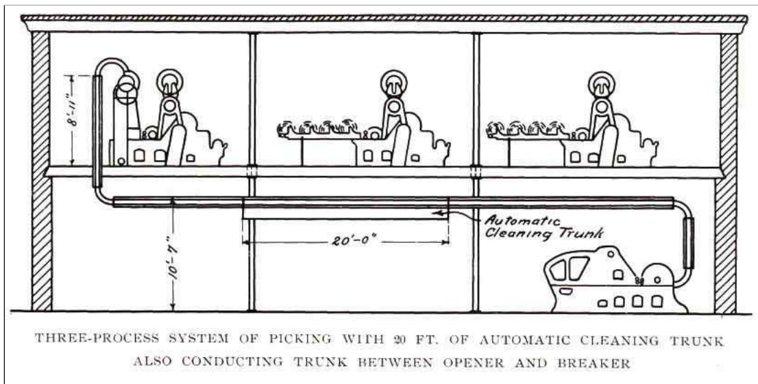
THREE-PROCESS SYSTEM OF PICKING WITH 20 FT. OF AUTOMATIC CLEANING TRUNK ALSO CONDUCTING TRUNK BETWEEN OPENER AND BREAKER
