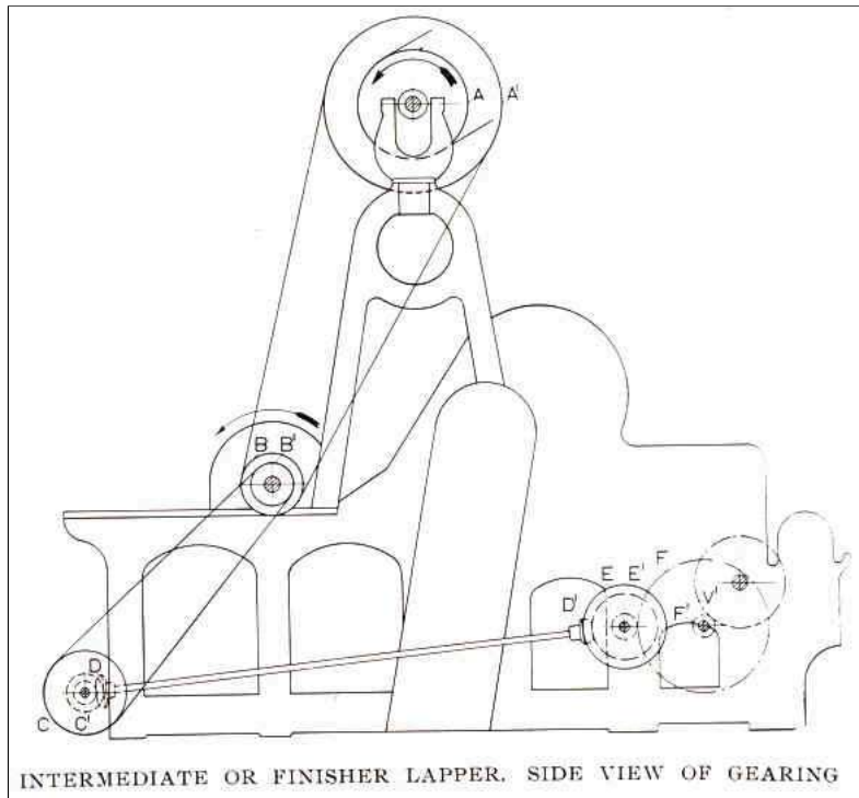
INTERMEDIATE OR FINISHER LAPPER. SIDE VIEW OF GEARING
