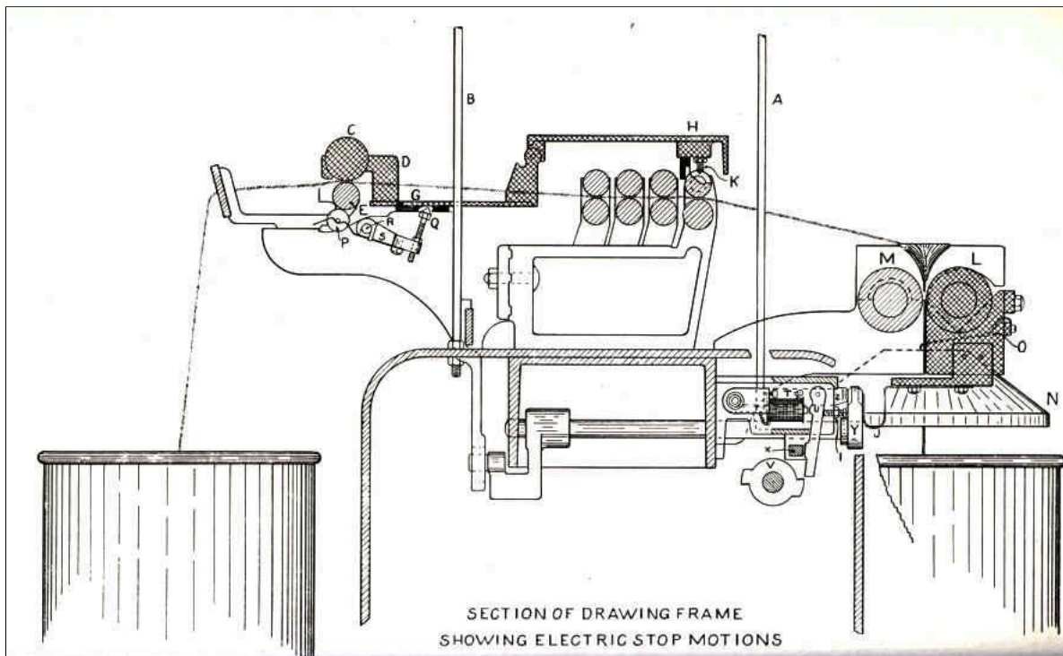
SECTION OF DRAWING FRAME
