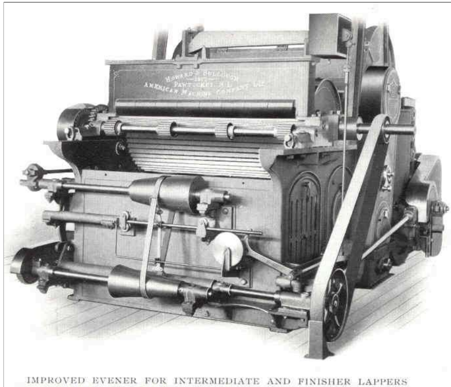
IMPROVED EVENER FOR INTERMEDIATE AND FINISHER LAPPERS
