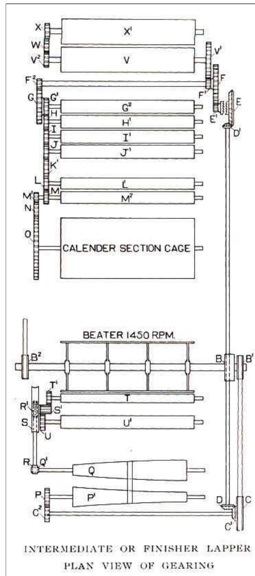
INTERMEDIATE OR FINISHER LAPPER PLAN VIEW OF GEARING
