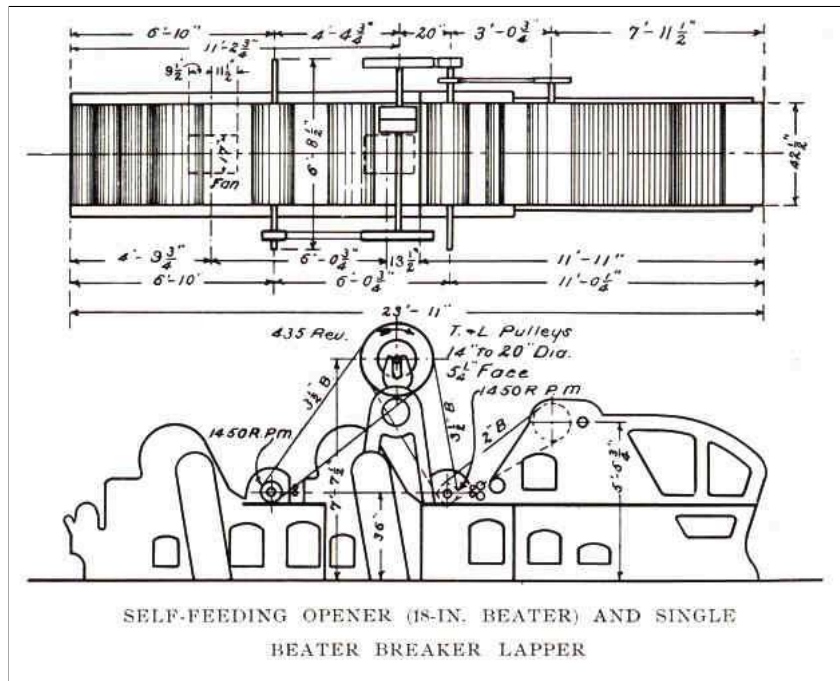
SELF-FEEDING OPENER (18-IN. BEATER) AND SINGLE BEATER BREAKER LAPPER
