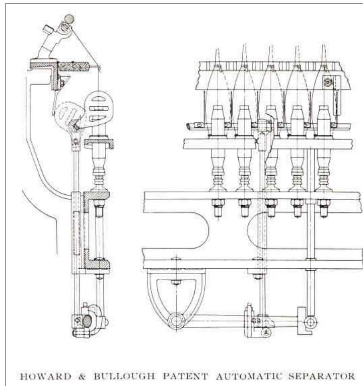
HOWARD &amp; BULLOUGH PATENT AUTOMATIC SEPARATOR
