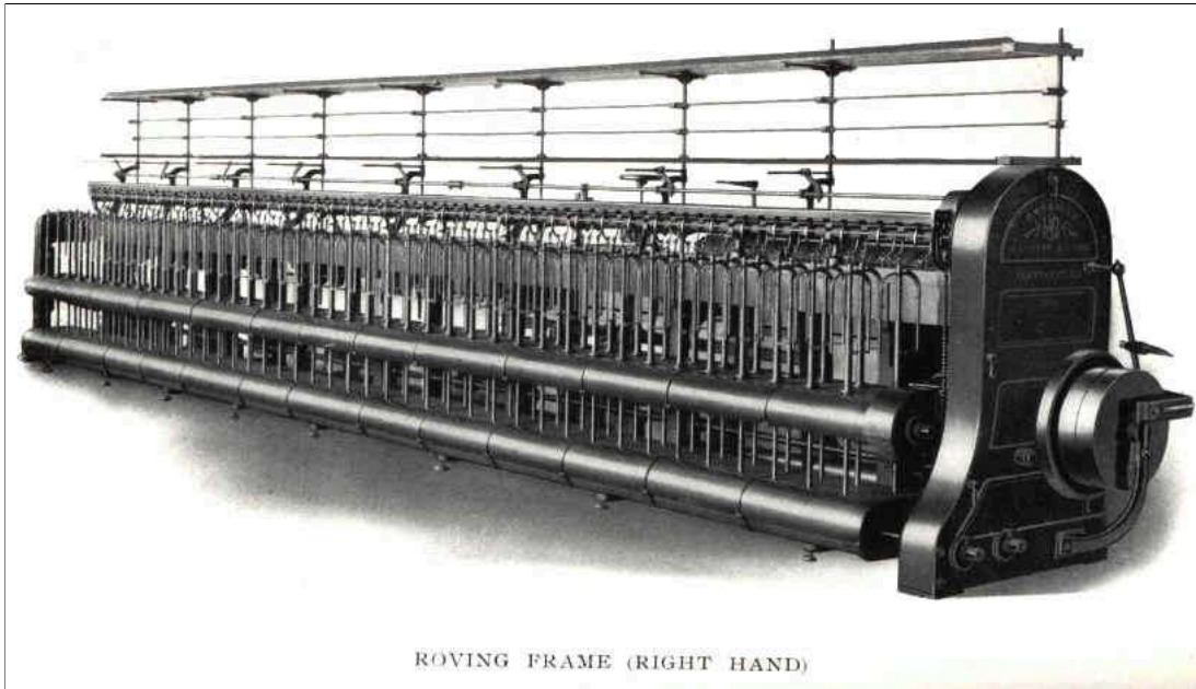
ROVING FRAME (RIGHT HAND)
