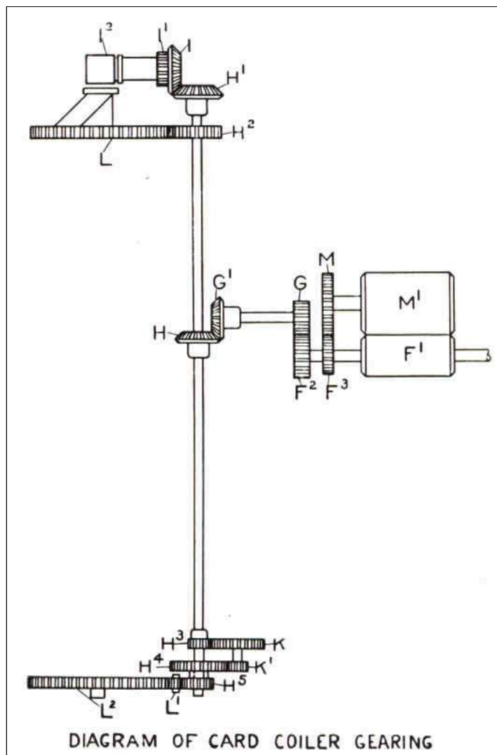
DIAGRAM OF CARD COILER GEARING
