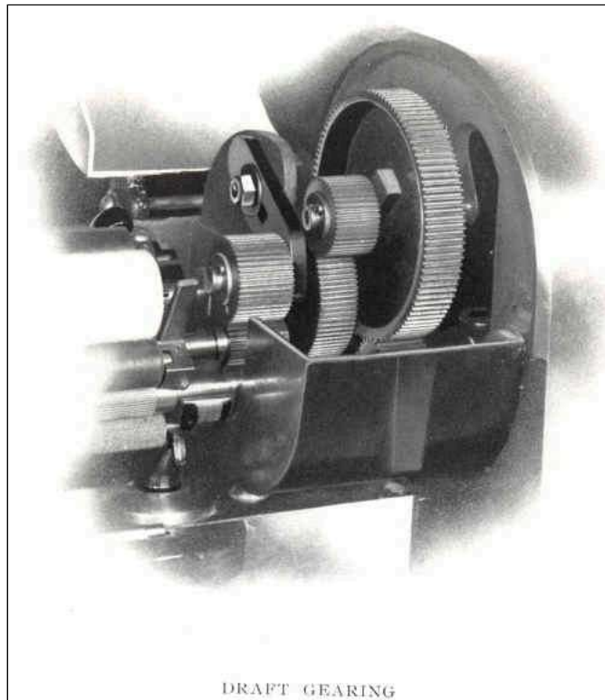
DRAFT GEARING DRAFT GEARING
