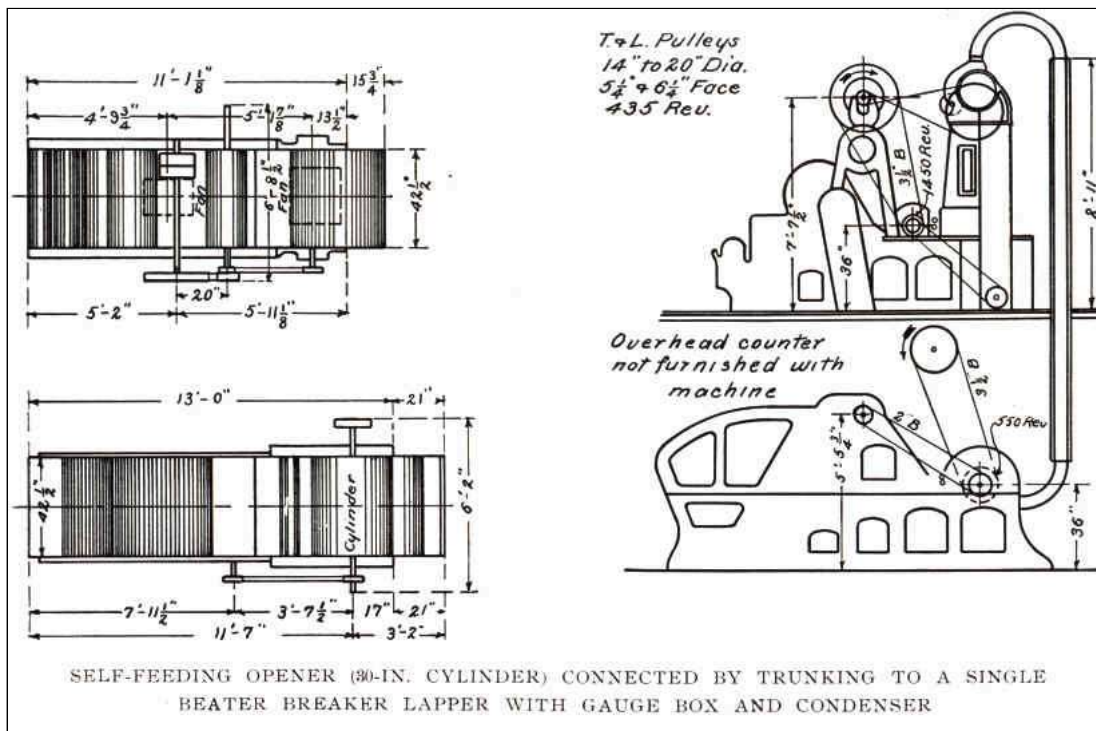
SELF-FEEDING OPENER (30-IN. CYLINDER) CONNECTED BY TRUNKING TO A SINGLE BEATER BREAKER LAPPER WITH GAUGE BOX AND CONDENSER
