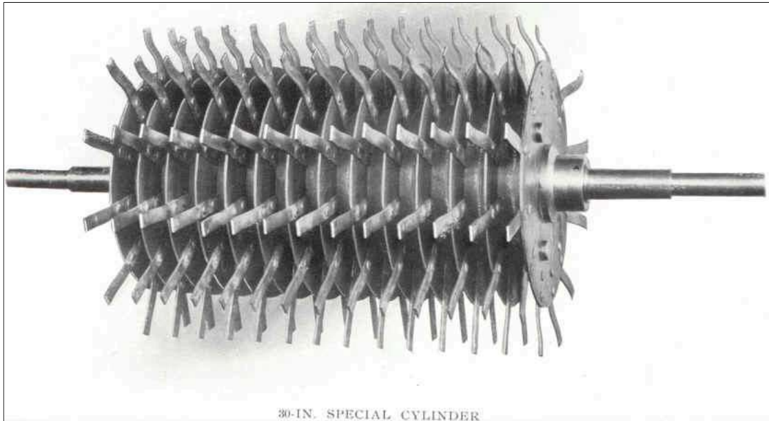
30-IN. SPECIAL CYLINDER 30-IN. SPECIAL CYLINDER
