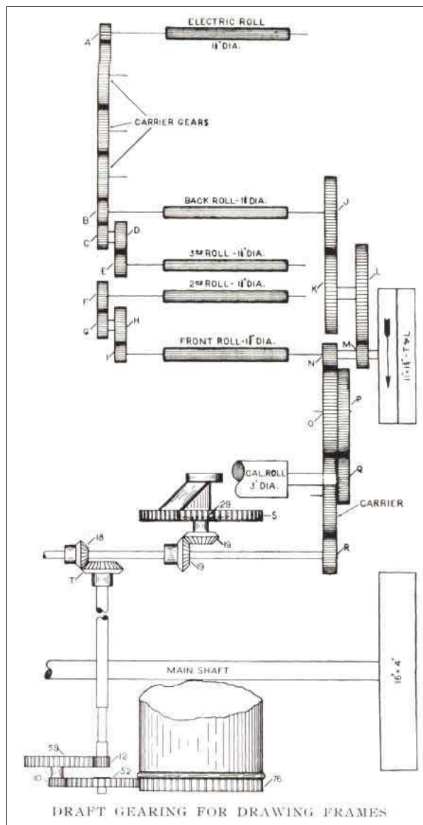
DRAFT GEARING FOR DRAWING FRAMES
